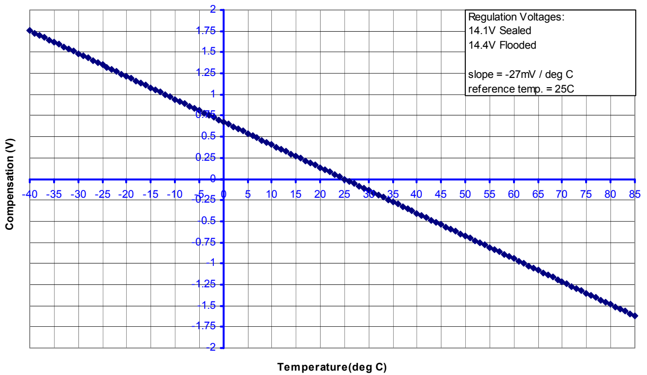
Temperature Compensation (SunLight 12V Models)
