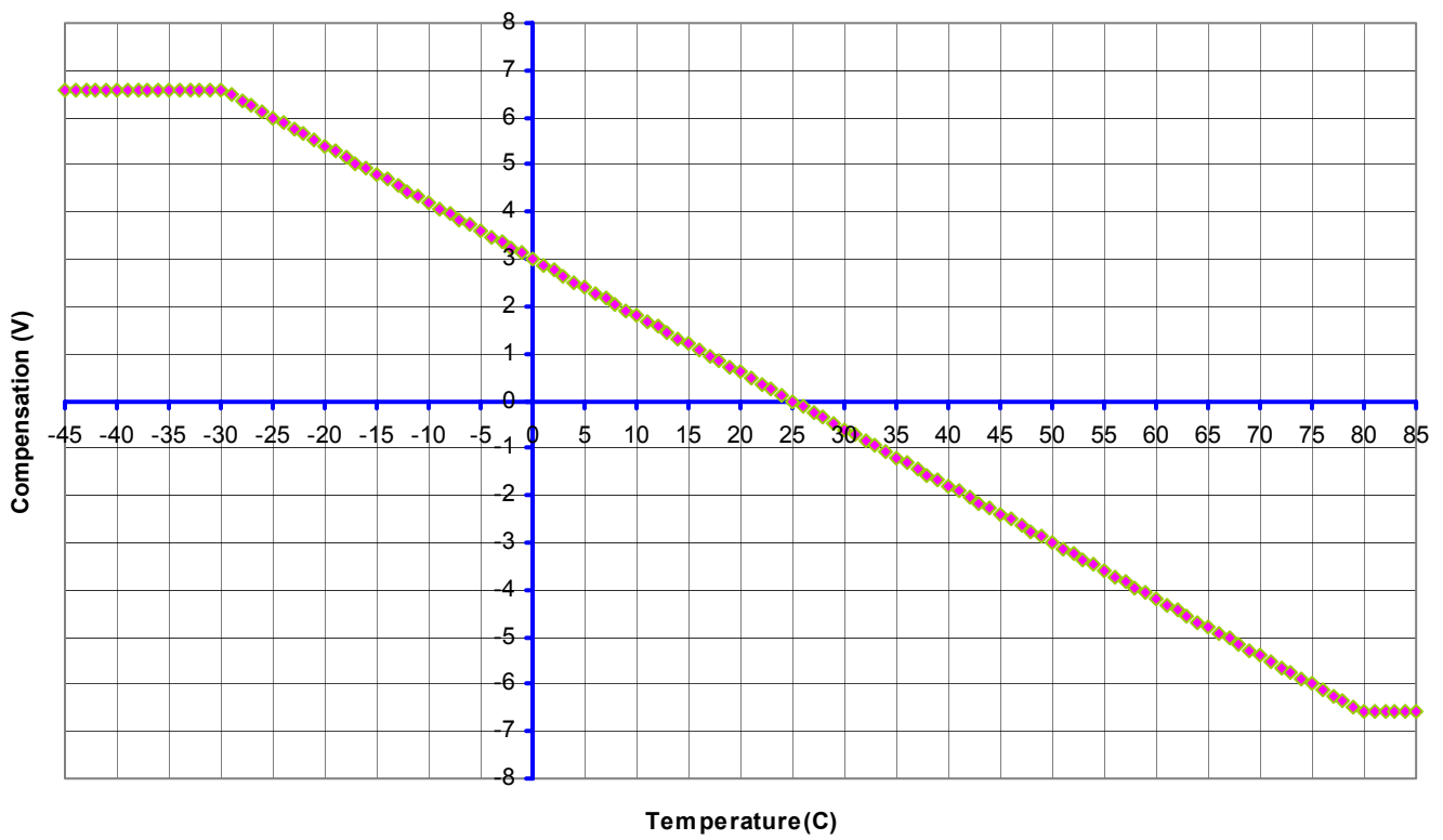
Temperature Compensation ProStar 48V
